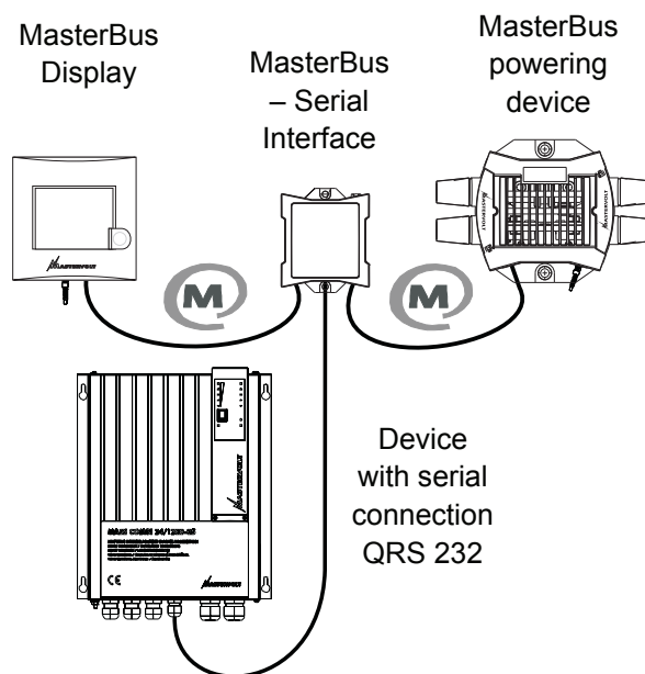
Figure 1: MasterBus-Serial interface in system
